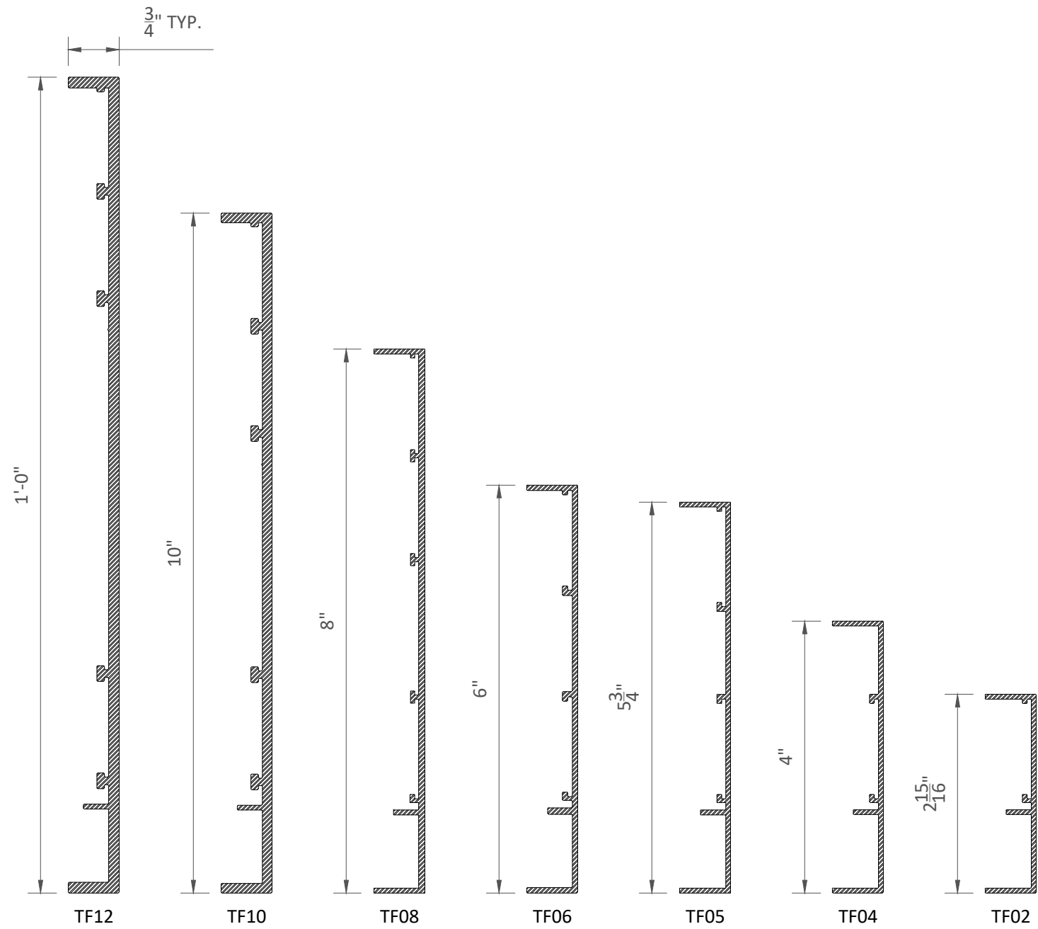
TF EDGELINE PROFILES
