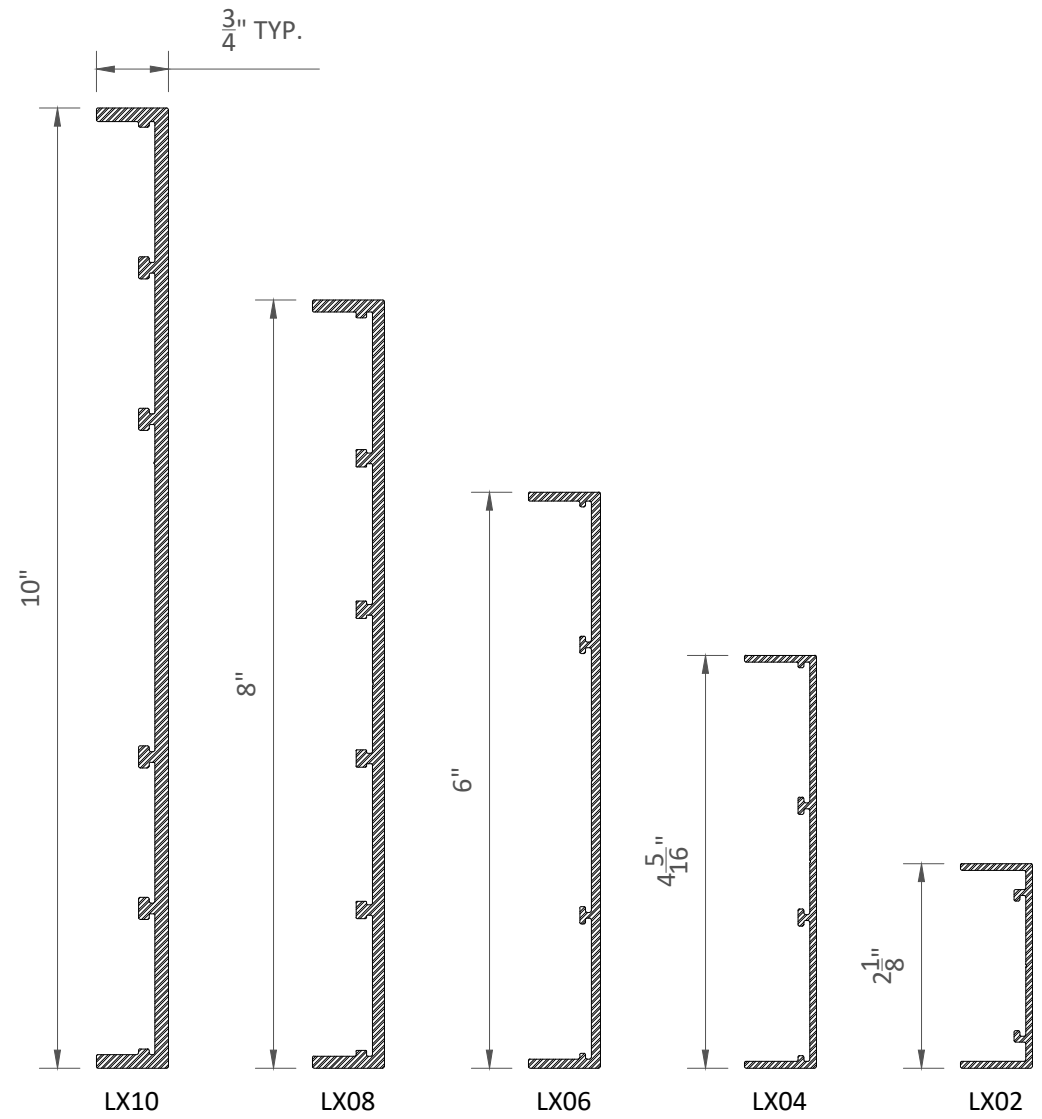
LX EDGELINE PROFILES
