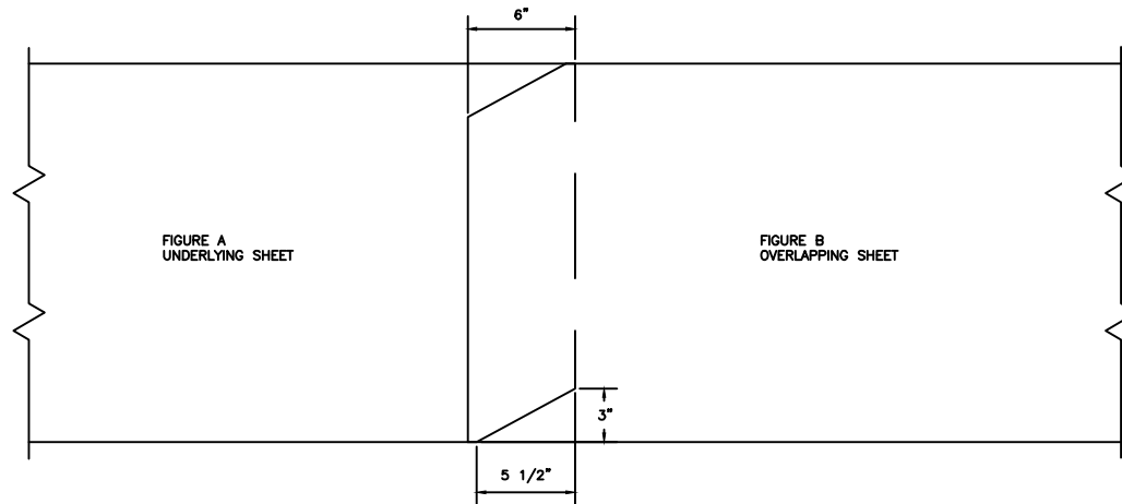
DIAGRAM 2. FINISHED END LAP DETAIL
