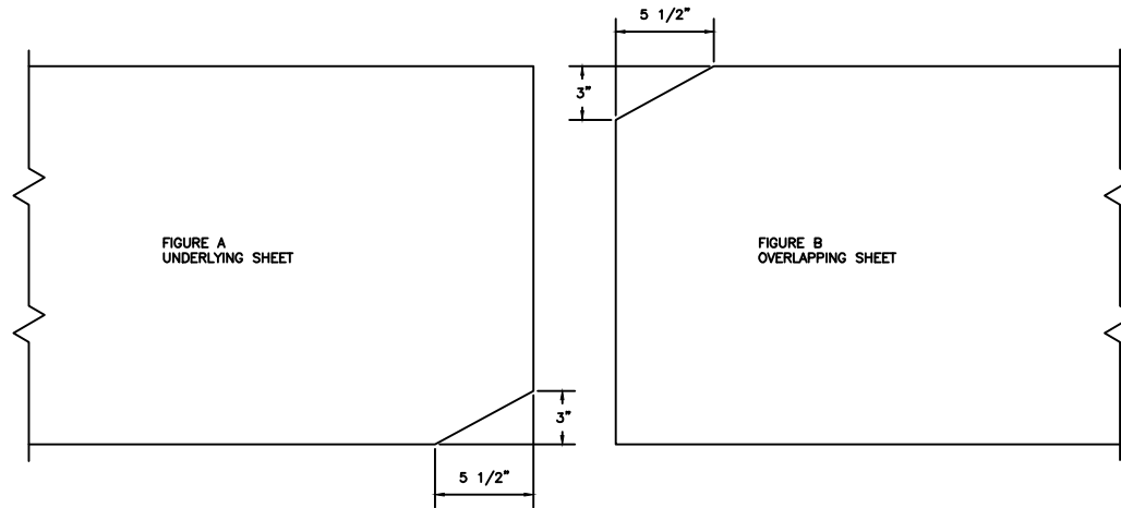
DIAGRAM 1. END LAP TRIM PATTERN BEFORE APPLICATION
